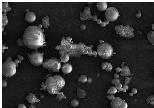
Figure 1. SEM image of class C fly ash.
