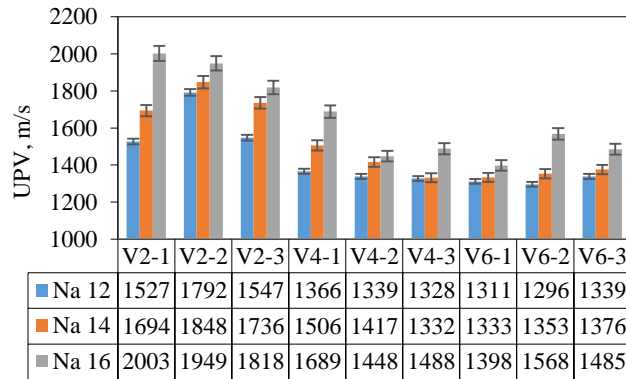
Figure 7. UPV values of the samples.
