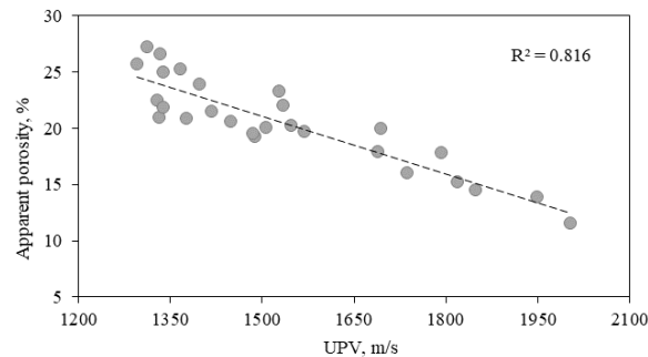
Figure 8. Relationship between apparent porosity and UPV.
