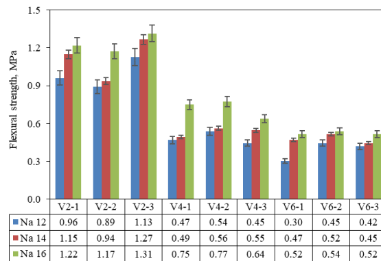
Figure 11. Flexural strength test results.
