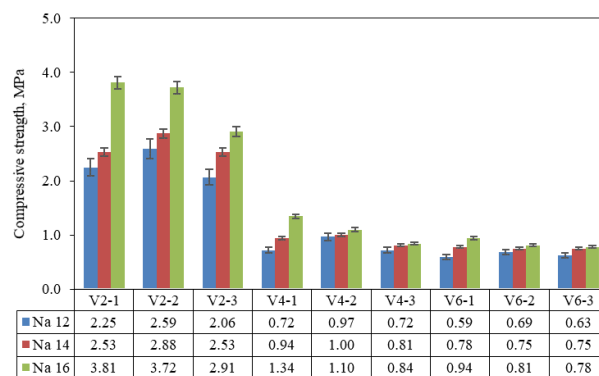
Figure 12. Compressive strength test results.
