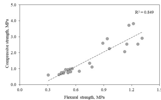
Figure 14. Relationship between flexural and compressive strengths.
