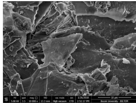
Figure 3. SEM image of expanded vermiculite.
