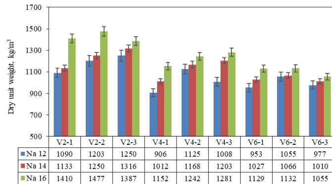
Figure 4. Dry unit weights of the samples.
