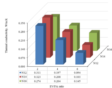
Figure 10. Thermal conductivity test results.
