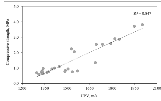
Figure 13. Relationship between UPV and compressive strength.
