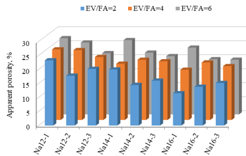
Figure 5. Apparent porosity test results.
