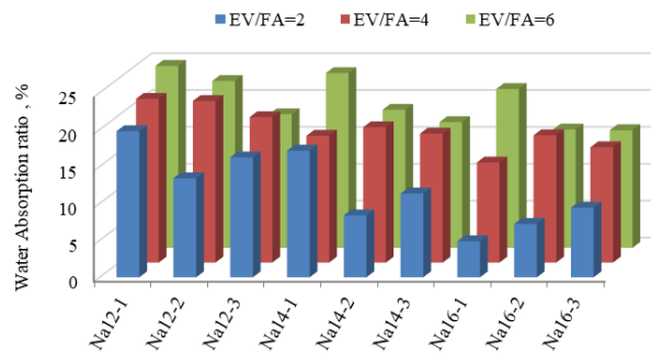
Figure 6. Water absorption ratio test results.
