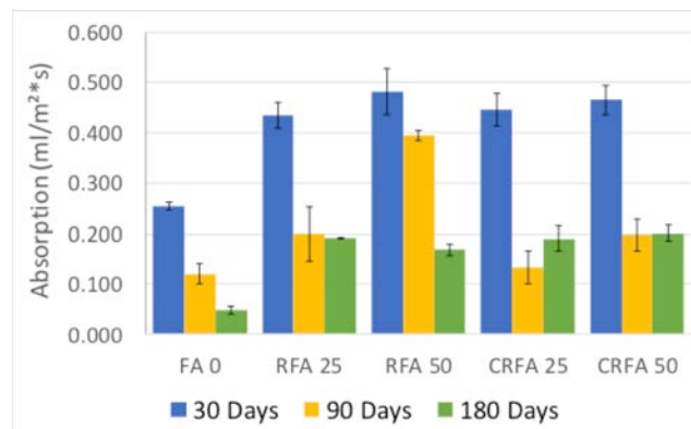
Figure 7. ISAT of the mortars after the initial 10 minutes of the test
